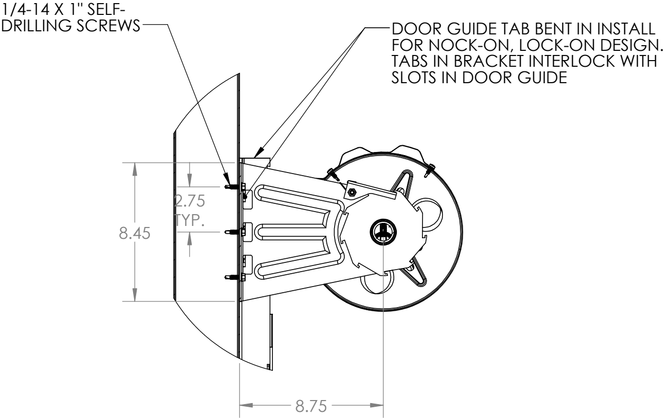
DOOR BRACKET TO STEEL JAMB
